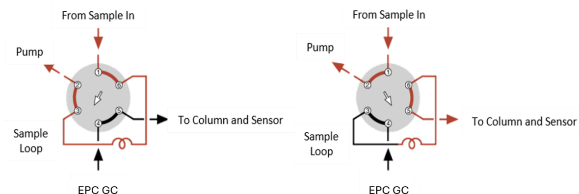
Figure 9: Six-Port Valve - Position Fill Loop and Inject
