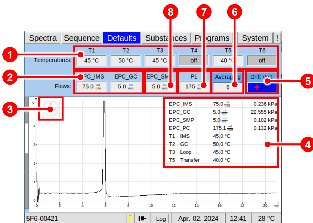
Figure 28: Operating Interface - Defaults Window
