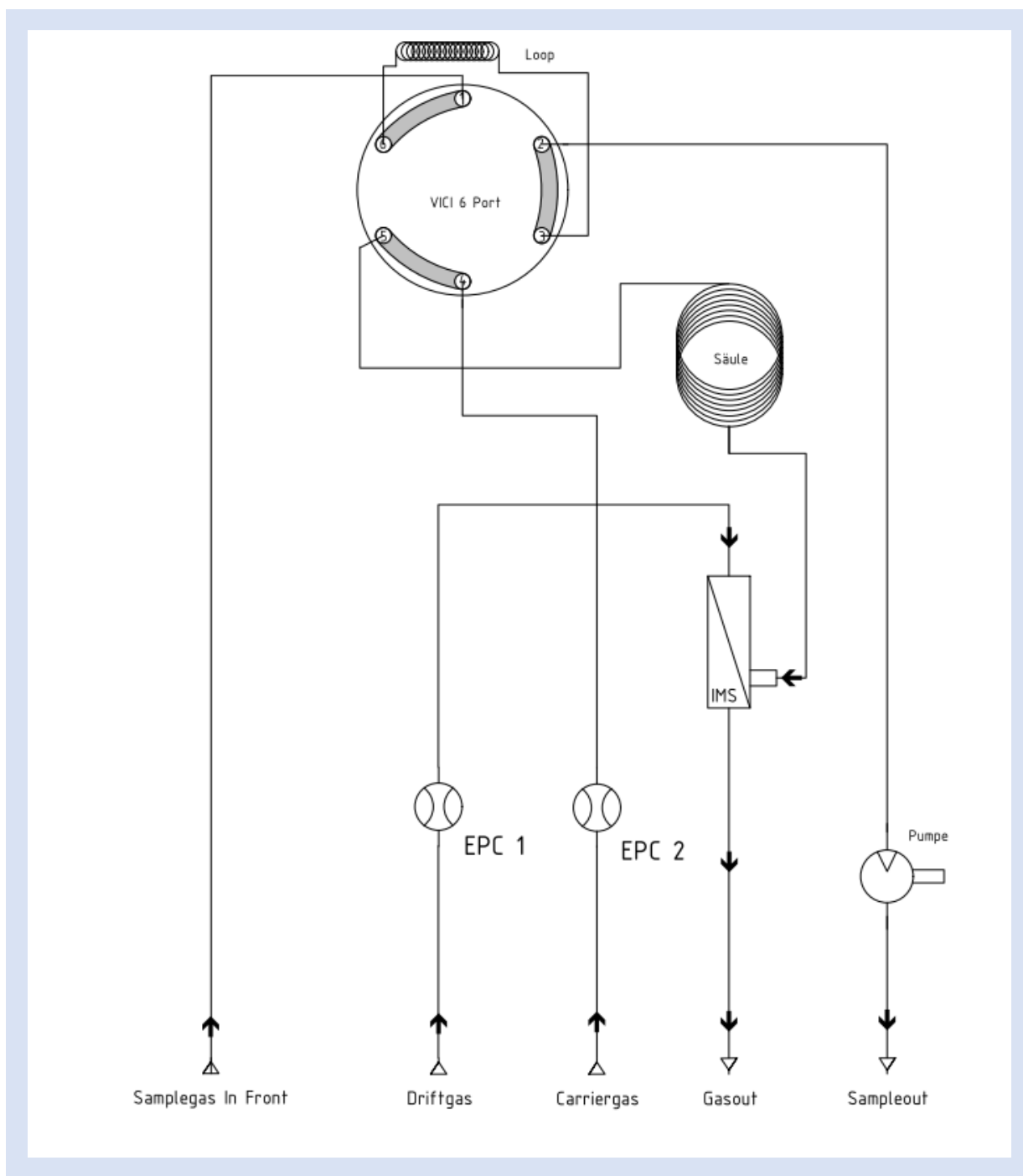
Figure 85: The gas flow diagram
