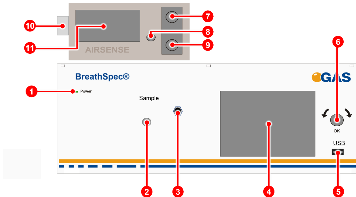
Figure 13: BreathSpec® (Version 5G2) with Airsense μTD - Housing of device - Front
