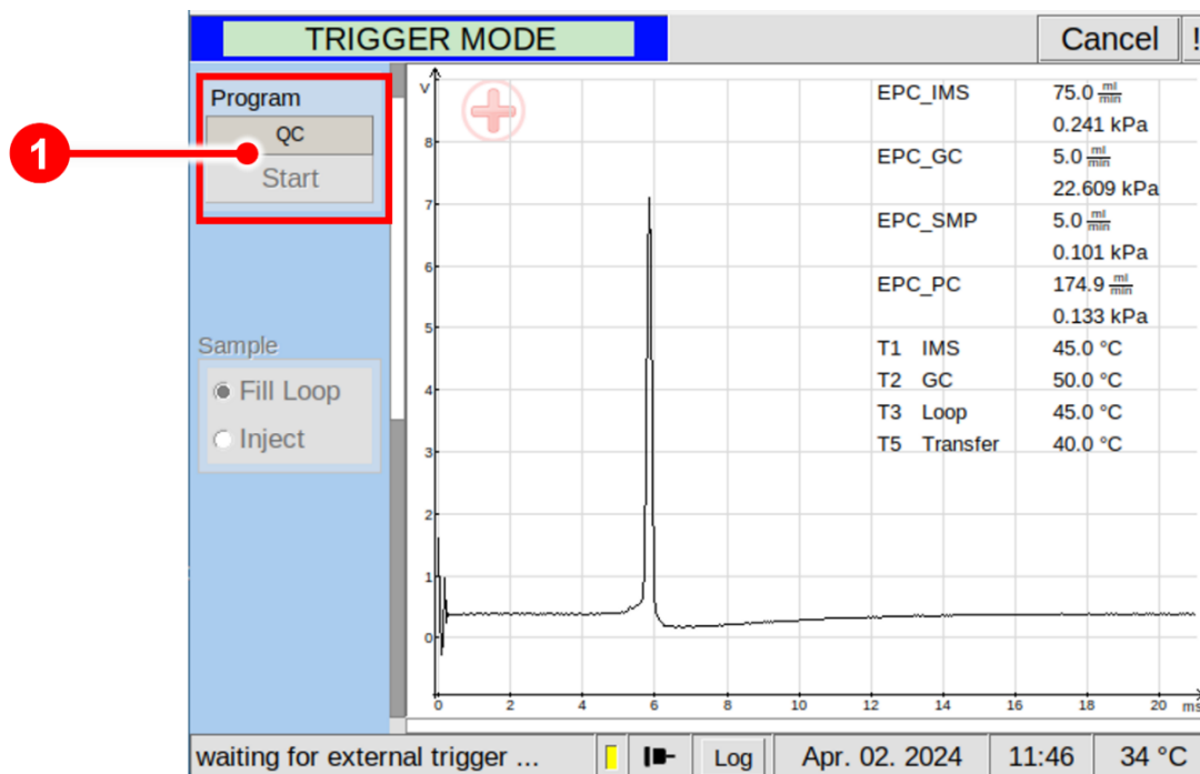
Figure 69: Operating Interface - Trigger Mode Window
