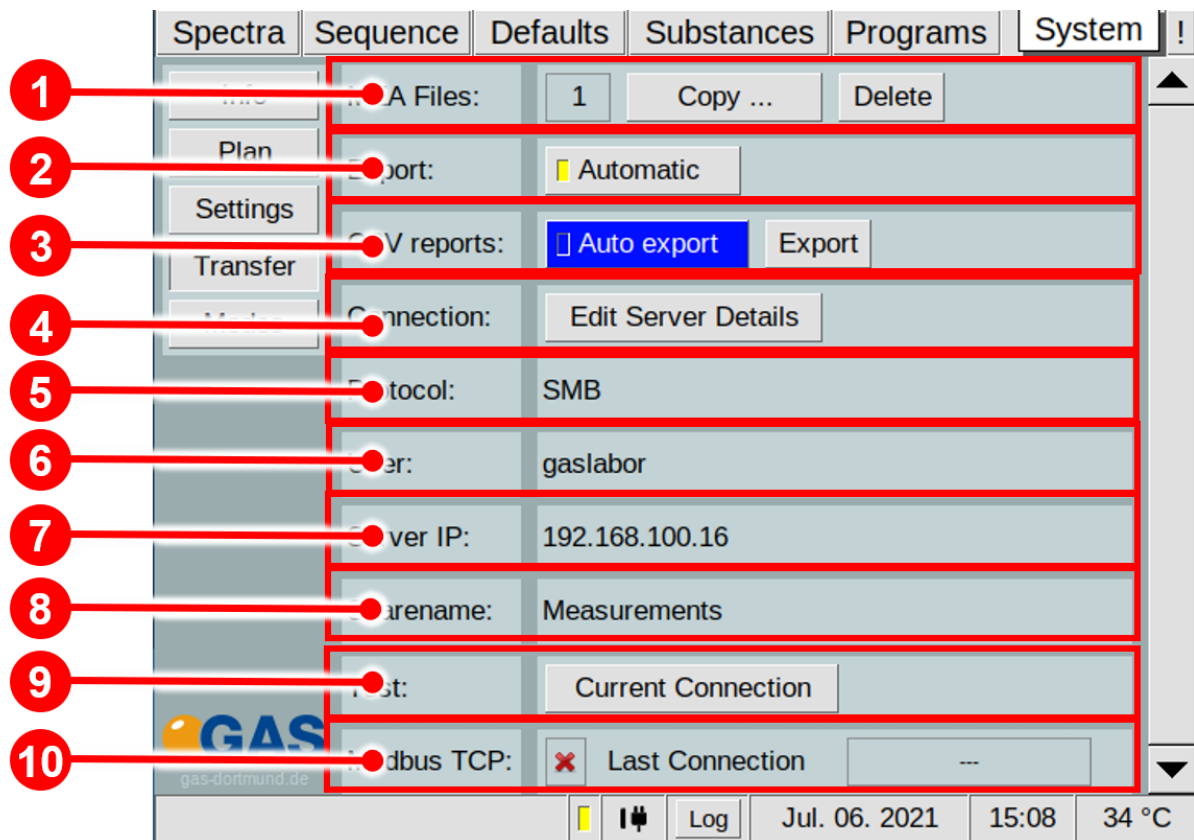
Figure 64: Operating Interface - System Transfer Window
