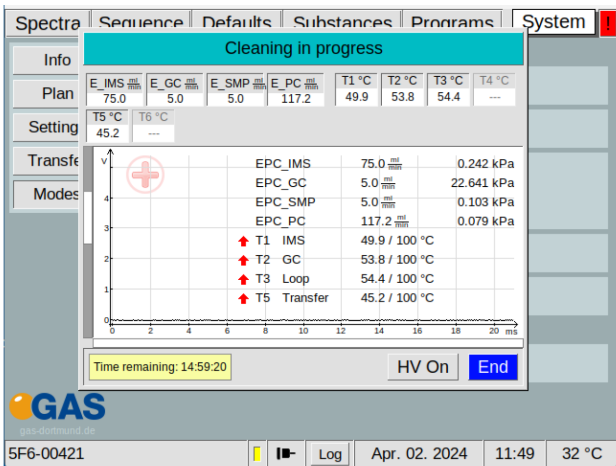
Figure 72: Operating Interface - Cleaning Mode Window
