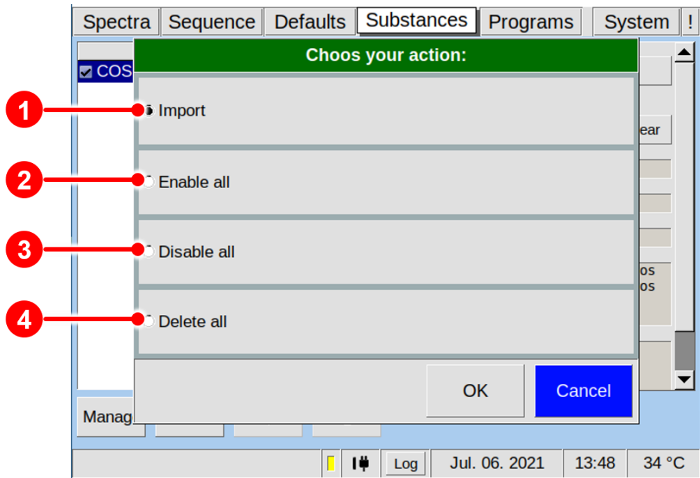
Figure 34: Substance List Control panel
