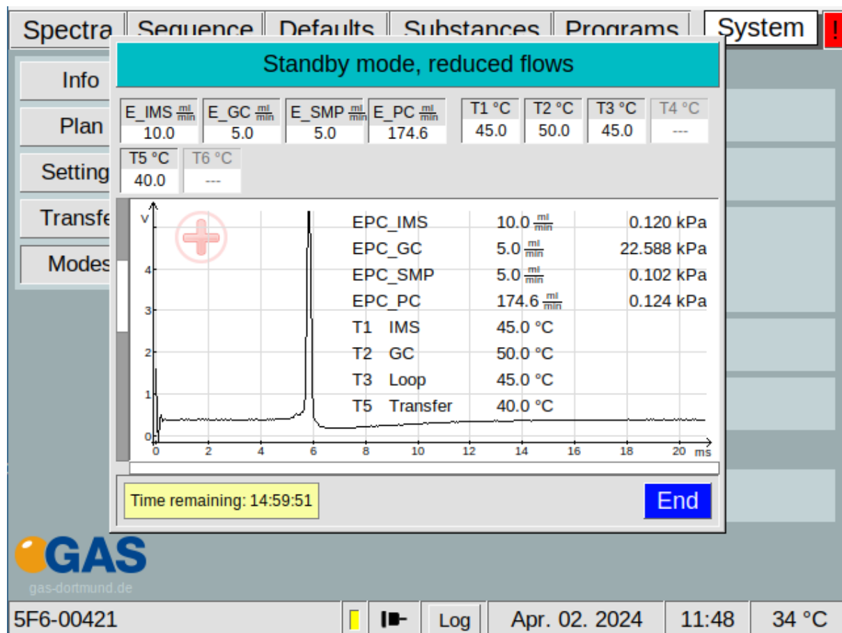
Figure 73: Operating Interface - Standby Mode Window
