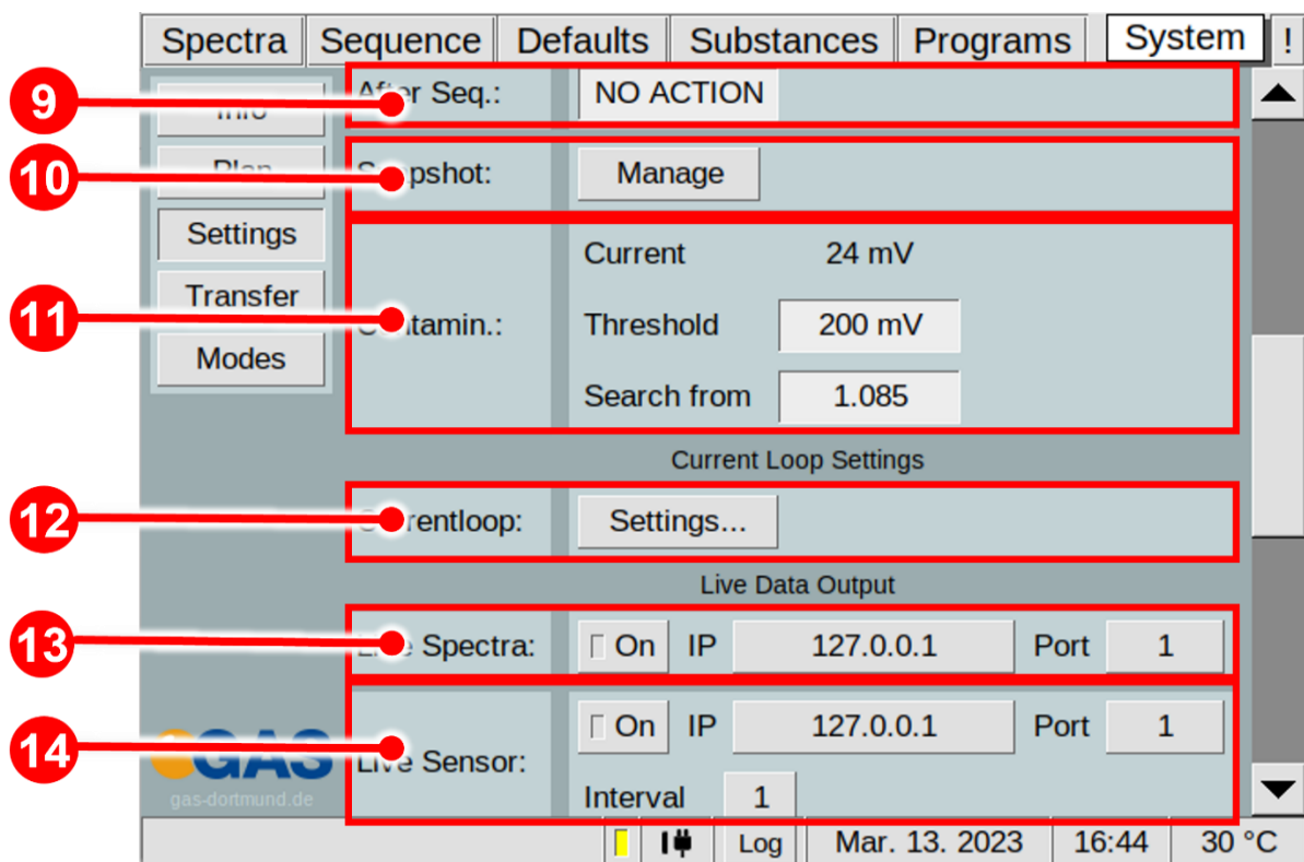
Figure 55: Operating Interface - System Settings Window 2
